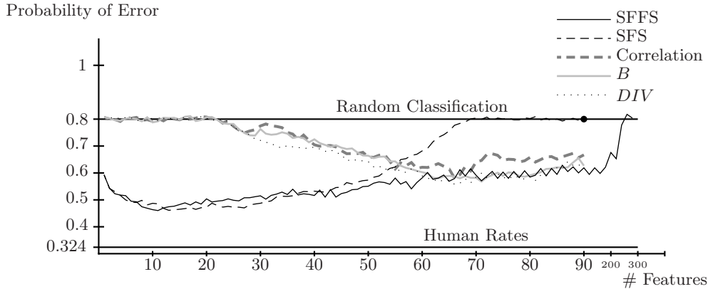
Fig. 1. Probability of classification error versus the number of features retained/discarded by feature selection method on DES.
